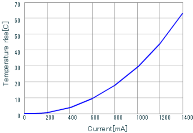
LQH2HPN6R8MJR DT_Current
