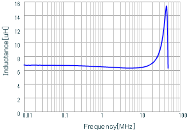
LQH2HPN6R8MJR L
