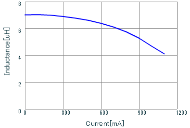
LQH2HPN6R8MJR DC-Bias, 20
