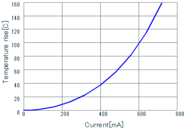
LQH3NPN680MGR DT_Current
