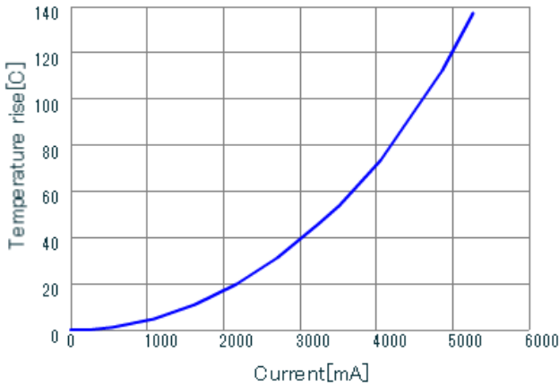
LQH5BPN2R7NT0 DT_Current
