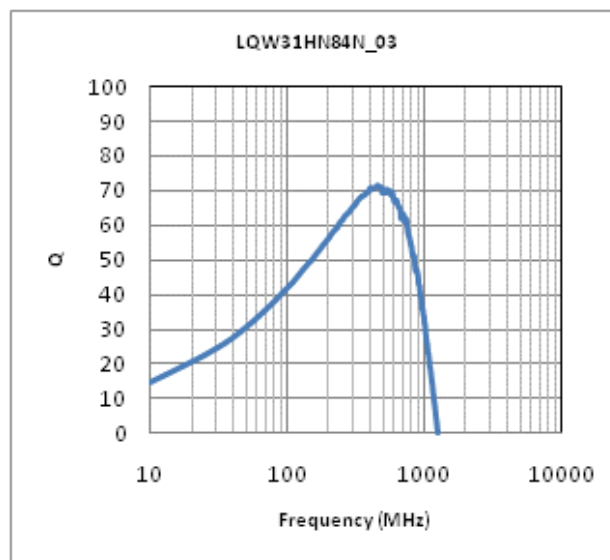
Q-Frequency Characteristics
