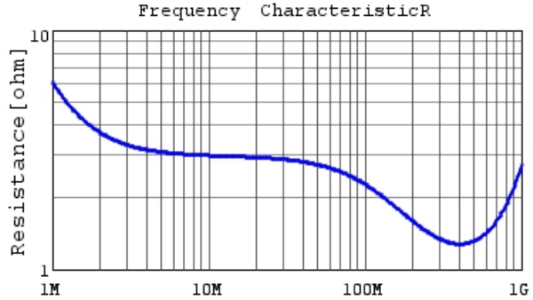
DE1B3RA101KJ4BP01F R DCOV, 20degC
