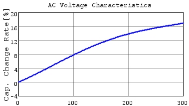
DE1B3RA101KJ4BP01F C-AC Voltage capchange, 1
