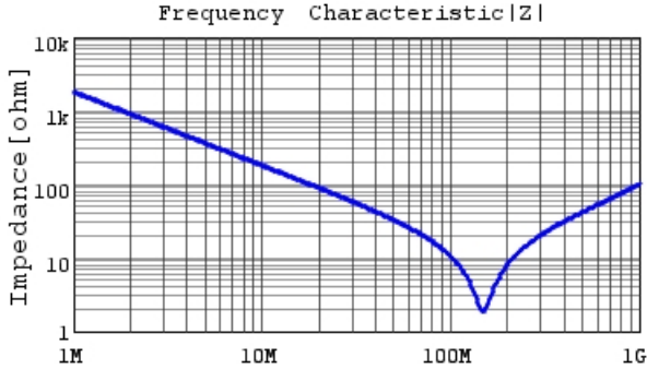
DE1B3RA101KJ4BP01F |Z| DCOV, 20degC
