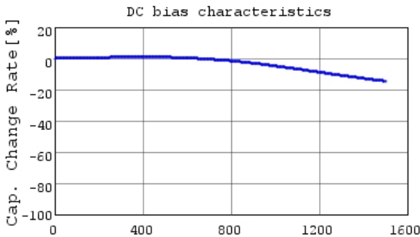
DE1B3RA101KJ4BP01F C-DC bias capchange, 20.0
