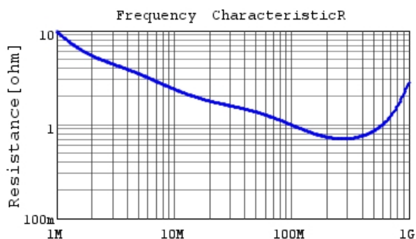
DE1B3RA471KA4BP01F R DCOV, 20degC
