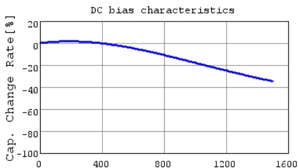
DE1B3RA471KA4BP01F C-DC bias capchange, 20.0
