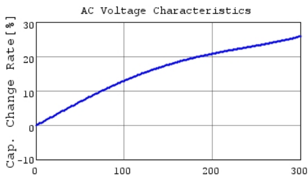
DE1B3RA471KA4BP01F C-AC Voltage capchange, 1
