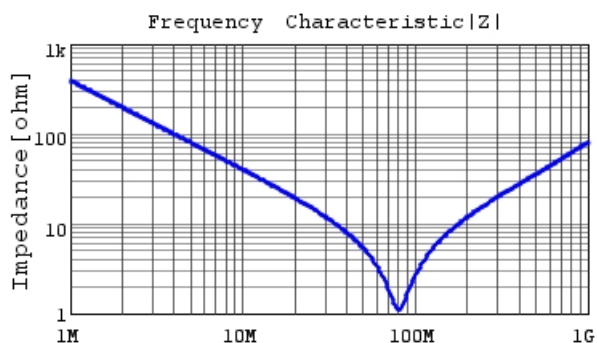
DE1B3RA471KA4BP01F |Z| DCOV, 20degC
