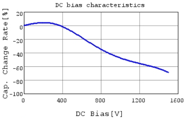
DE1E3RA152MN4AN01F C-DC bias capchange, 20.0
