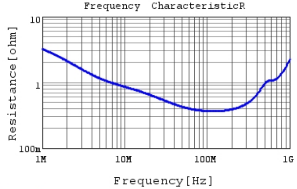
DE1E3RA152MN4AN01F R DCOV, 20degC
