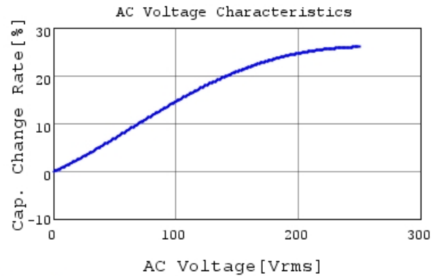
DE1E3RA152MN4AN01F C-AC Voltage capchange, 1
