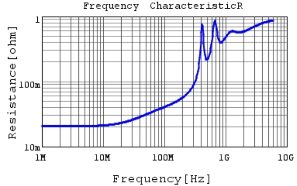
GRM1885C2A102JA01 R DCOV,25degC
