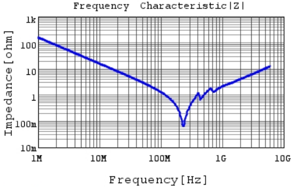
GRM1885C2A102JA01 |Z| DCOV,25degC
