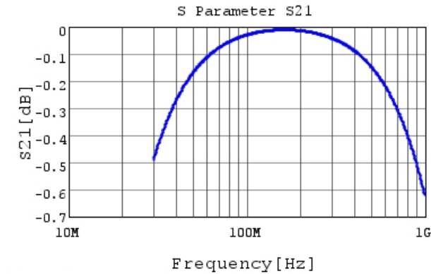
RHE5G1H151J0K1H03B S21 DCOV, 25degC
