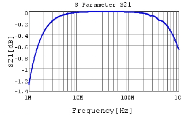
RHE5G1H272J0K1H03B S21 DCOV, 25degC
