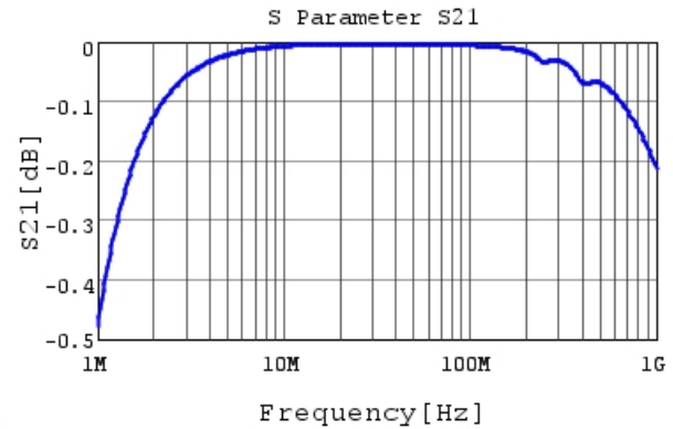
RHE5G1H472J1DBH03A S21 DCOV, 25degC
