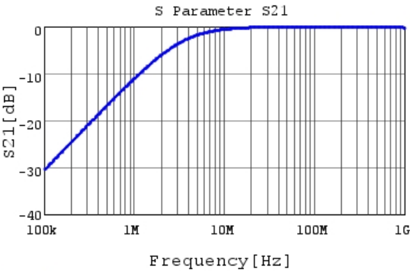
RHEL81H471K0DBH03A S21 DCOV, 25degC
