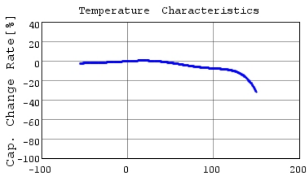
■ RHEL81H684K2M1H03A C-Temp. capchange, DCOV,
