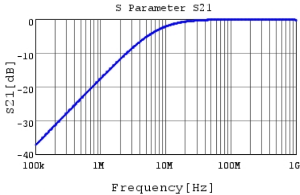
RHEL82A221K0DBH03A S21 DCOV, 25degC
