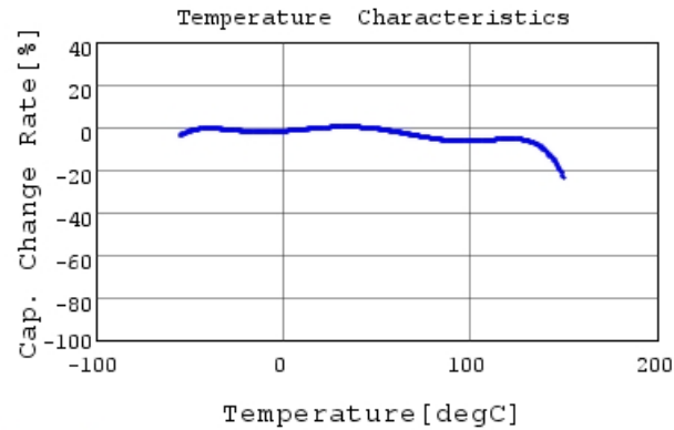
RHEL82A222K0A2H03B C-Temp. capchange, DCOV,
