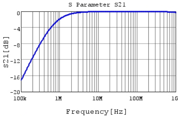
RHEL82A222K0A2H03B S21 DCOV, 25degC
