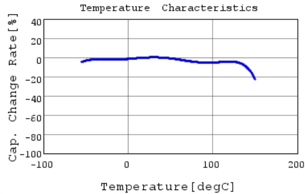
RHEL82A681K0A2H03B C-Temp. capchange, DCOV,
