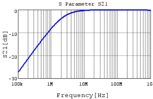
RHEL82A681K0A2H03B S21 DCOV, 25degC
