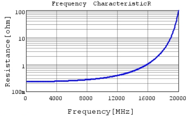
GJM1555C1H1R0BB01 R DCOV,25degC
