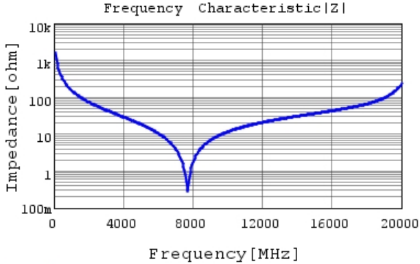
GJM1555C1H1R0BB01 |Z| DCOV,25degC
