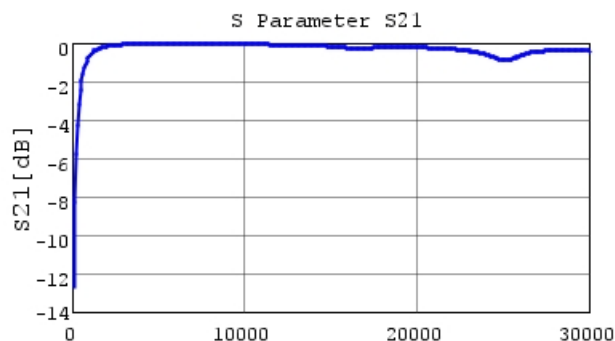
GRM0225C1H3R8BA03 S21 DCOV, 25degC
