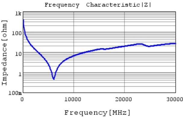
GRM0225C1H4R1BA03 |Z| DCOV,25degC
