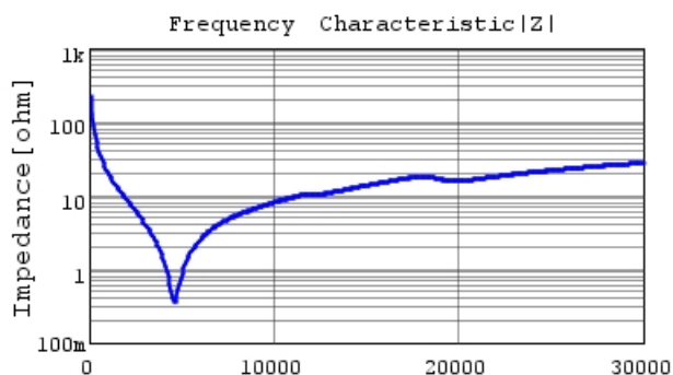
GRM0225C1H7R3DA03 |Z| DCOV,25degC
