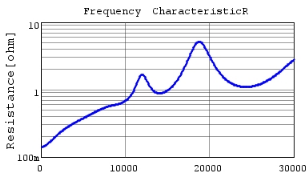
GRM0225C1H7R3DA03 R DCOV,25degC
