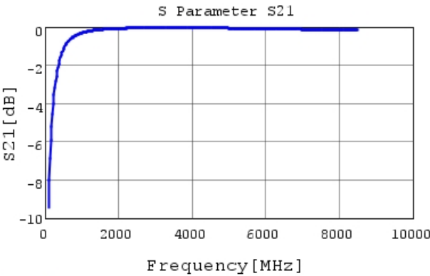
GRM0335C1H5R7WA01 S21 DCOV, 25degC
