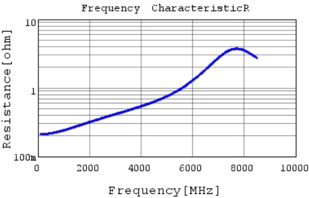
GRT1555C1H6R0DA02 R DCOV,25degC
