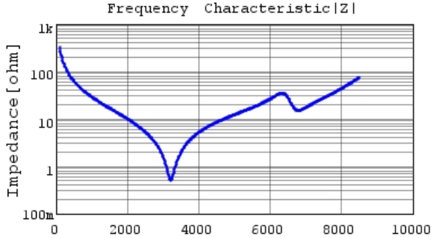
■ GRT1885C2A5R0CA02 |Z| DCOV, 25degC
