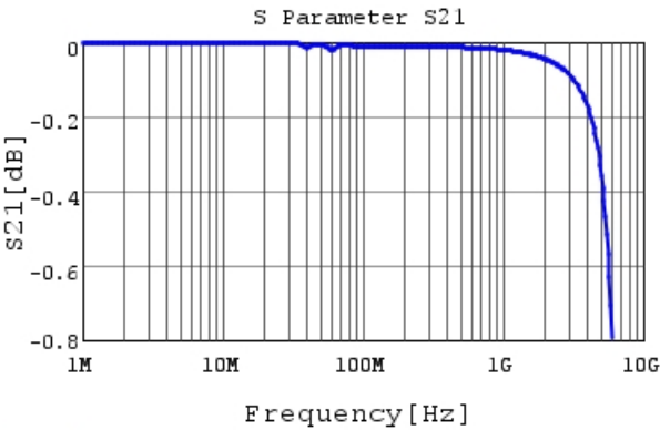
GRT31C5C1H683JA02 S21 DCOV, 25degC
