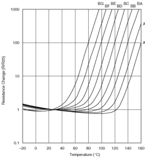
Resistance-Temperature Characteristics
