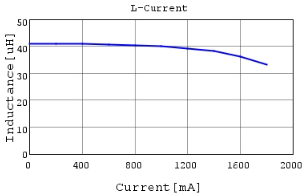
B1047AS-390M L-Current 20degC
