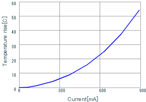
LQH2HPN150MJR DT_Current
