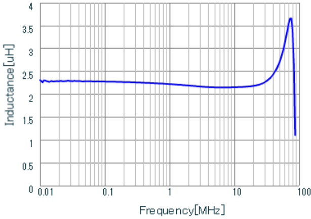
LQH2HPN2R2MJR L
