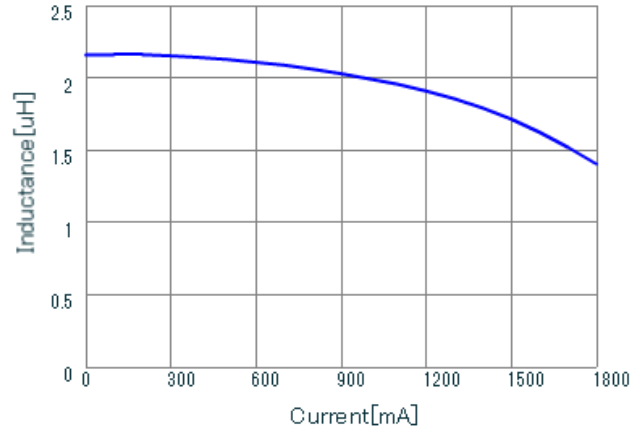
LQH2HPN2R2MJR DC-Bias, 20
