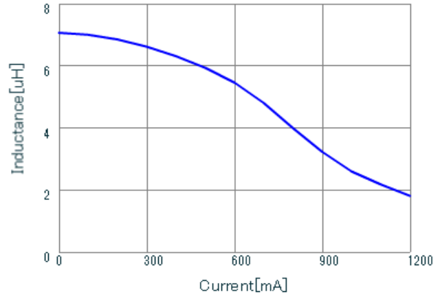
LQH3NPZ6R8MGR DC-Bias, 20
