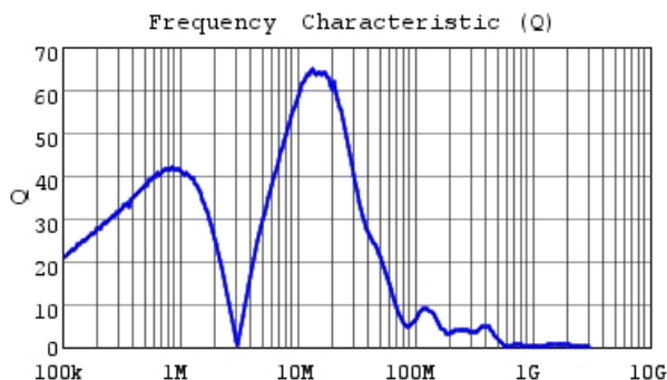
LQH43NZ102J03 Q
