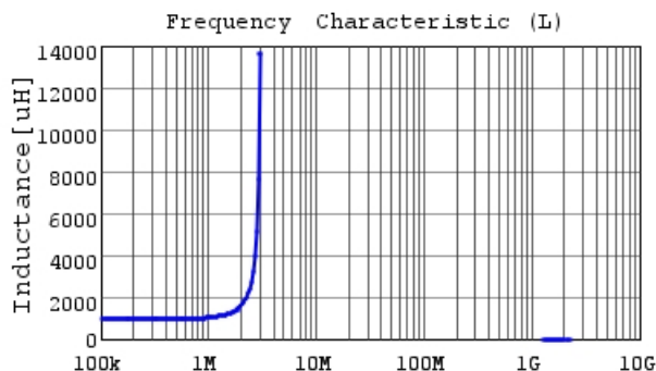
LQH43NZ102J03 L
