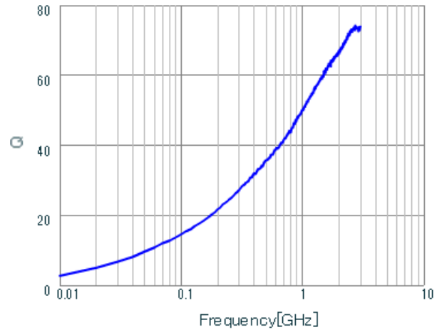
LQP03HQ3N0B02 Q.
