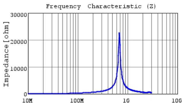
LQP03HQR43J02 |Z|
