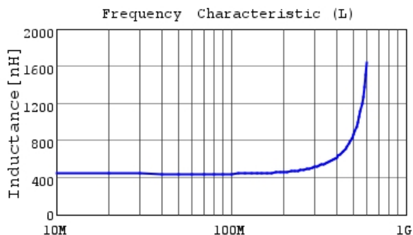
LQP03HQR43J02 L
