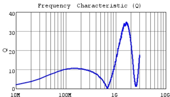
LQP03HQR43J02 Q
