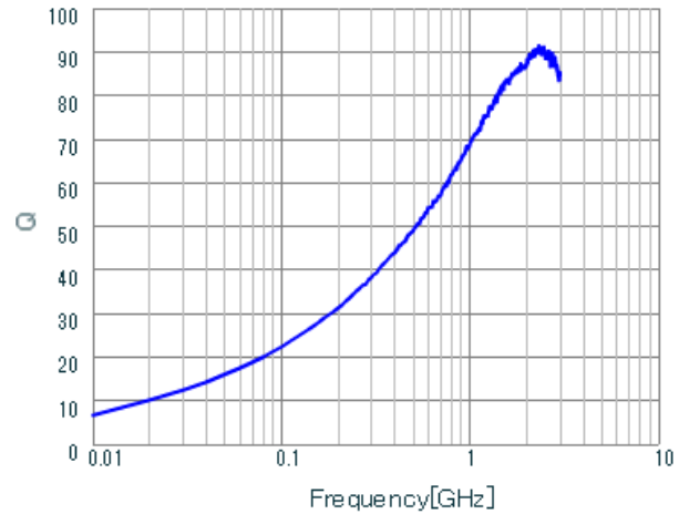
LQW15AN12NJ00 Q.
