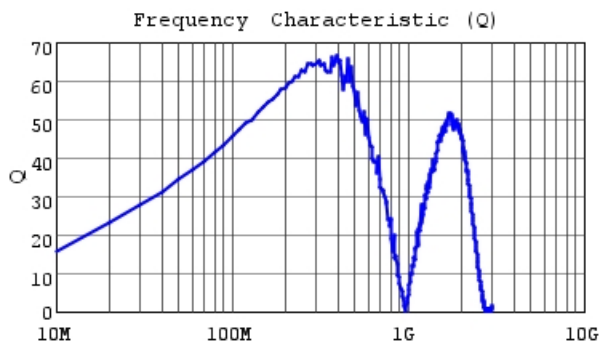
LQW2BASR24G00 Q
