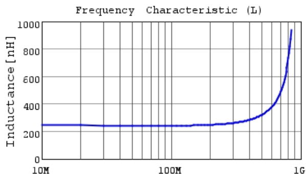
LQW2BASR24G00 L
