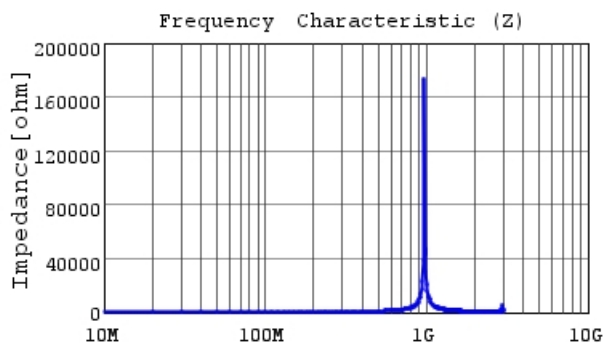
LQW2BASR24G00 |Z|
