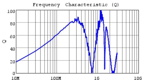
LQW2UASR27J00 Q
