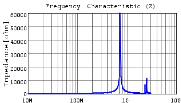
LQW2UASR27J00 |Z|
