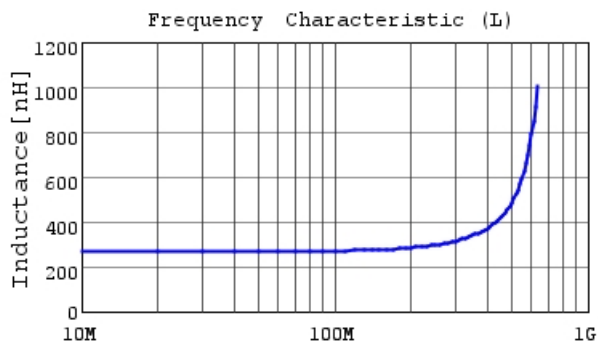
LQW2UASR27J00 L
