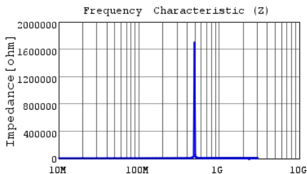
LQW2UASR62F00 |Z|
