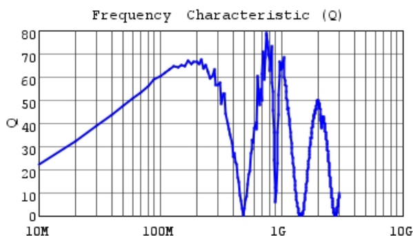
LQW2UASR62F00 Q
