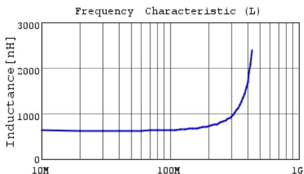
LQW2UASR62F00 L
