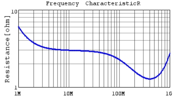
DE1B3RA101KA4BP01F R DCOV, 20degC
