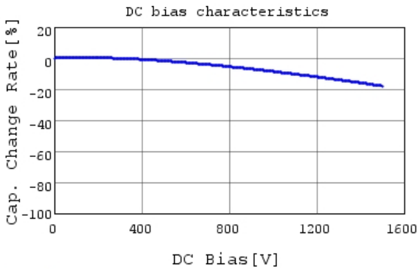
DE1B3RA101KA4BP01F C-DC bias capchange, 20.0
