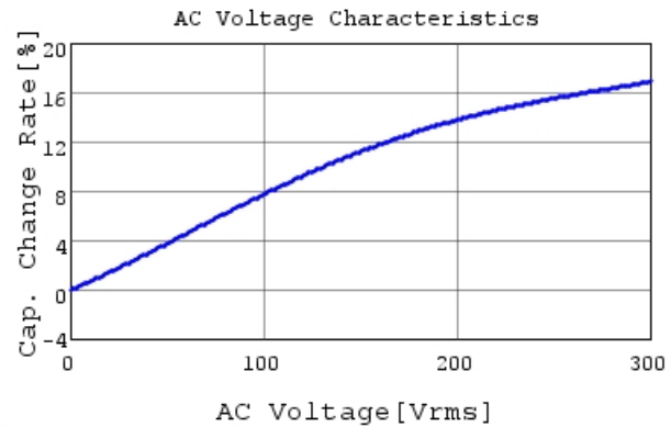
DE1B3RA101KA4BP01F C-AC Voltage capchange, 1
