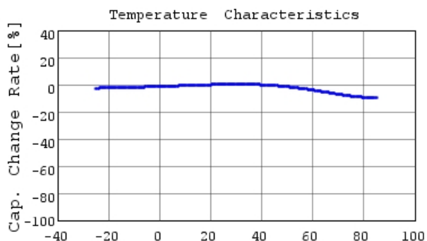
DE1B3RA331KJ4BP01F C-Temp. capchange, DCOV,
