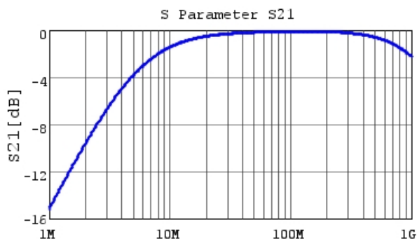
DE1B3RA331KJ4BP01F S21 DCOV, 20degC
