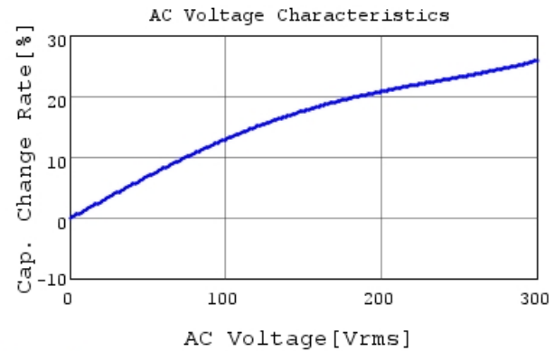
DE1B3RA471KA4BP01F C-AC Voltage capchange, 1
