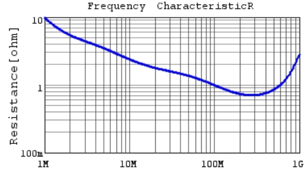
DE1B3RA471KA4BP01F R DCOV, 20degC
