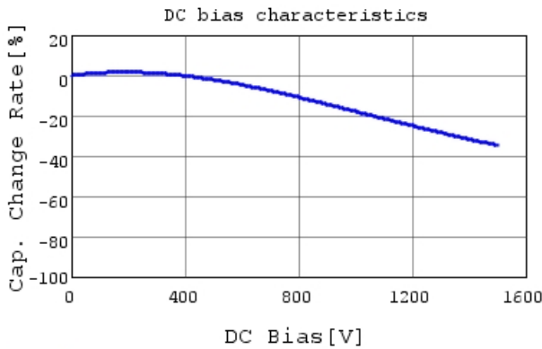
DE1B3RA471KA4BP01F C-DC bias capchange, 20.0
