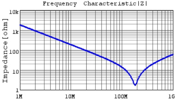
DE2B3SA101KA2BT01F |Z| DCOV, 20degC
