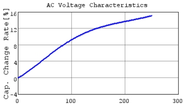
DE2B3SA101KA2BT01F C-AC Voltage capchange, 1
