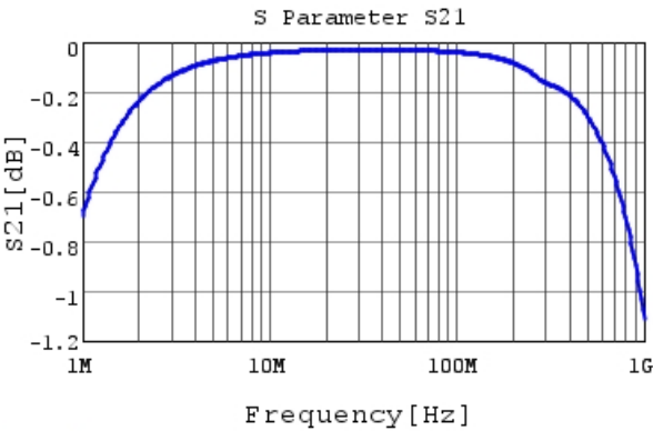
DE2E3KY472MA3BM02F S21 DC0V, 20degC
