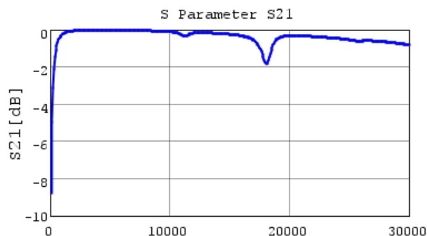
■ GJM0335C1E6R2CB01 S21 DCOV, 25degC
