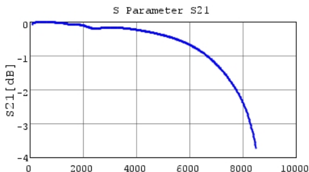
GRM1885C1H121JA01 S21 DCOV, 25degC
