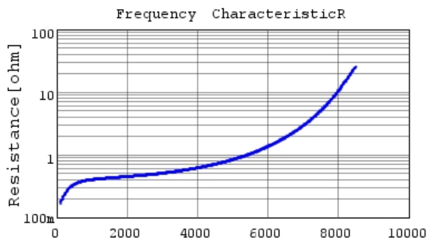
GRM1885C1H2R7CA01 R DCOV,25degC
