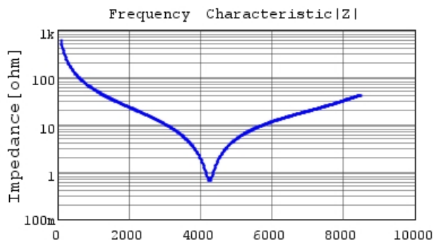
GRM1885C1H2R7CA01 |Z| DCOV,25degC
