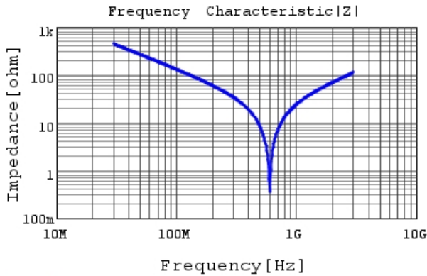
RCE5C3A120J2K1H03B |Z| DCOV, 25degC
