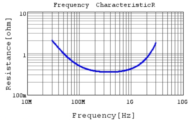
RCE5C3A120J2K1H03B R DCOV, 25degC
