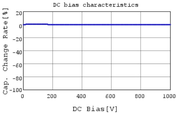
RCE5C3A120J2K1H03B C-DC bias capchange, 25.0
