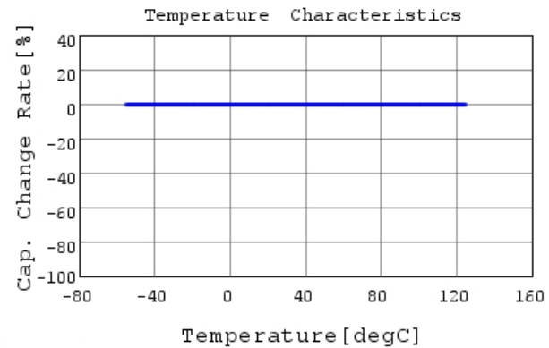
RCE5C3A120J2K1H03B C-Temp. capchange, DCOV,
