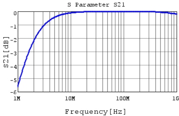
RHE5G1H102J0A2H03B S21 DCOV, 25degC
