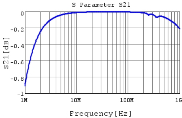
RHE5G1H332J0DBH03A S21 DCOV, 25degC
