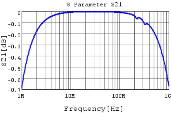
RHE5G1H392J0M1H03A S21 DCOV, 25degC
