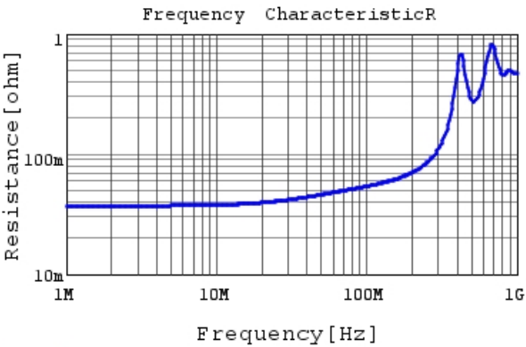
RHE5G2A102J0A2H03B R DCOV, 25degC
