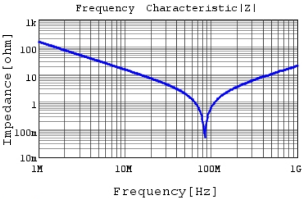
RHE5G2A102J0A2H03B |Z| DCOV, 25degC
