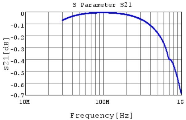
RHE5G2A391J0K1H03B S21 DCOV, 25degC
